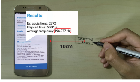
Fig. 7. Experimental Setup.
