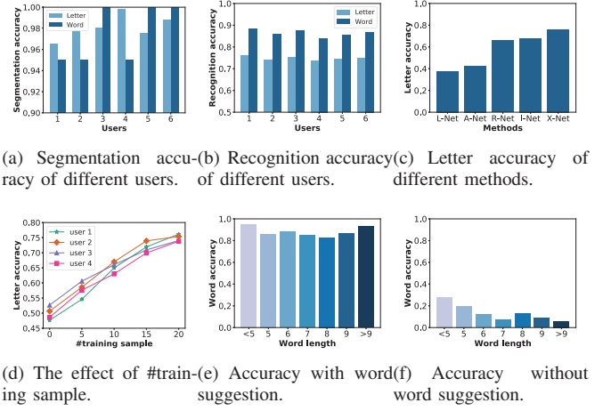
Fig. 8. Accuracy of the VibWriter system.
