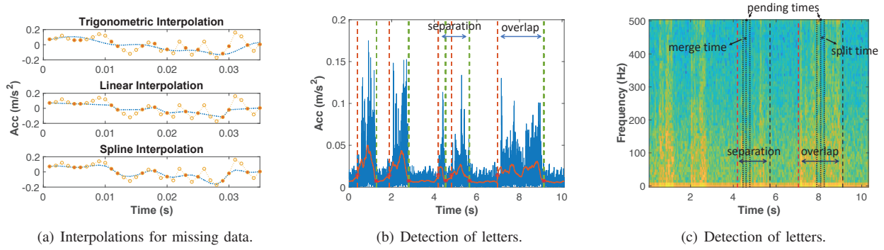
Fig. 4. Letter segmentation metrics: 4(a) Results of various interpolation methods: the red dots are the vibration signals (hollow dots are stable samples, solid dots are unstable samples), the blue lines are the interpolation results; 4(b) Vibration signal (blue) and corresponding weighted mean signal (red) showing different writing conditions: normal fast writing, an interruption during fast writing (with an interval during one letter) and continuous writing (without interval between letters). The dotted line indicates the results of segmentation based on amplitude; 4(c) Proposed solution to deal with signal separation and overlap caused by interruption and continuous writing.
