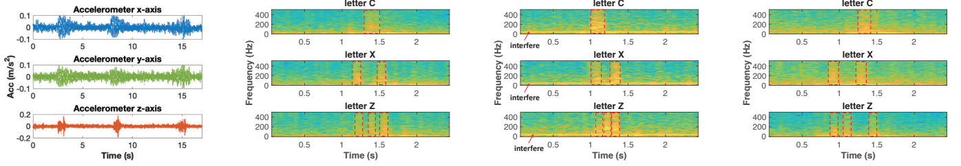
(a) Vibration signal of volunteer 1. (b) Frequency spectrum of volunteer 1. (c) Frequency spectrum of volunteer 1 with interferences. (d) Frequency spectra of volunteer 2.
