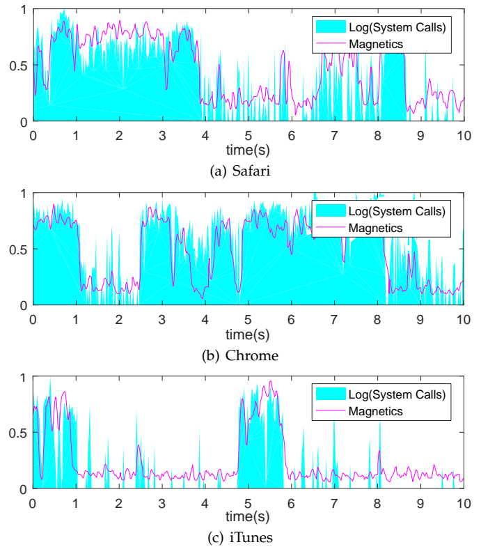
Fig. 2: EM signals are correlated with the system call traces but distinct among applications. Note that the two traces are normalized for illustration and the Y-axis represents the frequency of system calls or the magnitude of EM signals.
